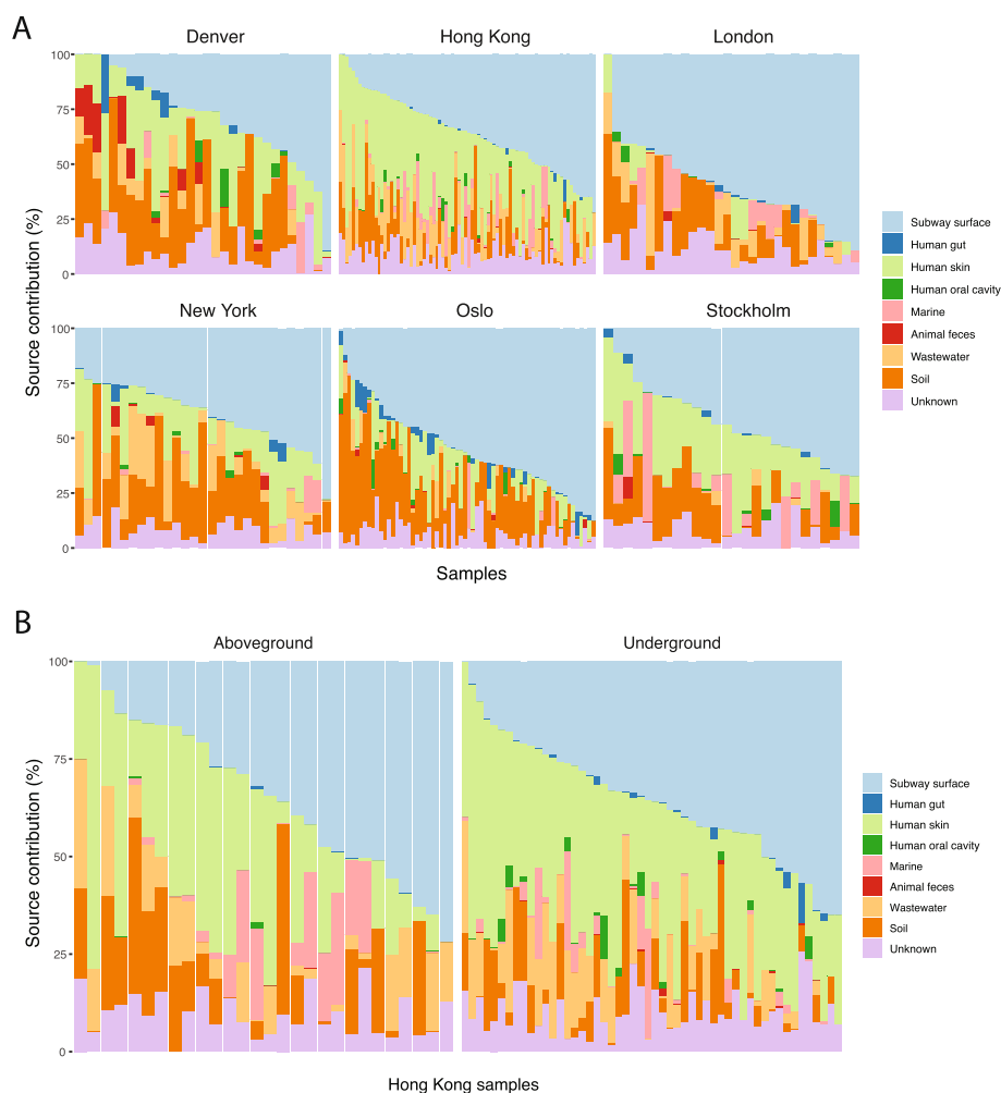
Fig. 5 Bayesian source tracking estimated public transit surface, human skin, and soil as major AR sources for public transit air resistome. Estimated proportions of resistome sources of different ecotypes in the public transit air microbiomes faceted by city (a) and by above- and underground stations within the Hong Kong public transit system (b)
