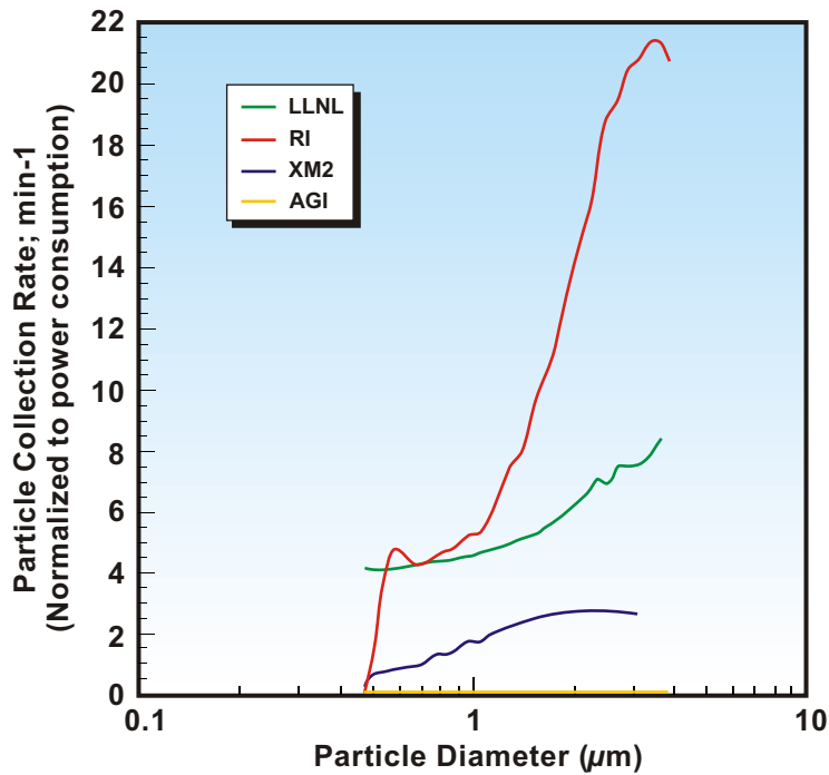
Collection efficiency for various samplers; normalized for power consumption.
