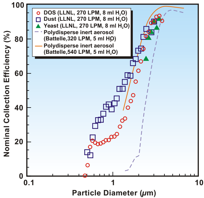
Collection efficiency for various particle types at low aerosol concentration.
